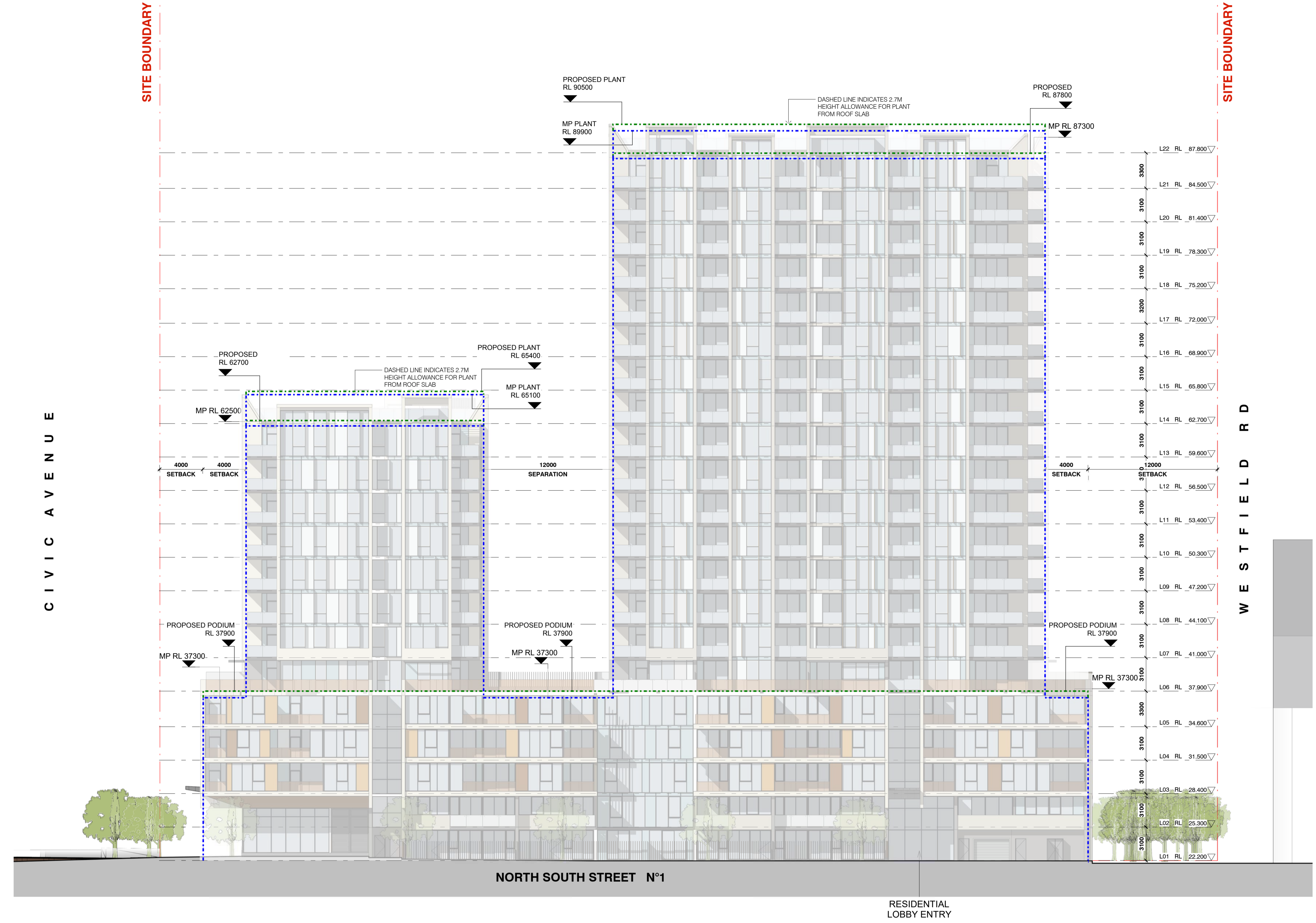
1 ELEVATION - WEST 1 : 200
