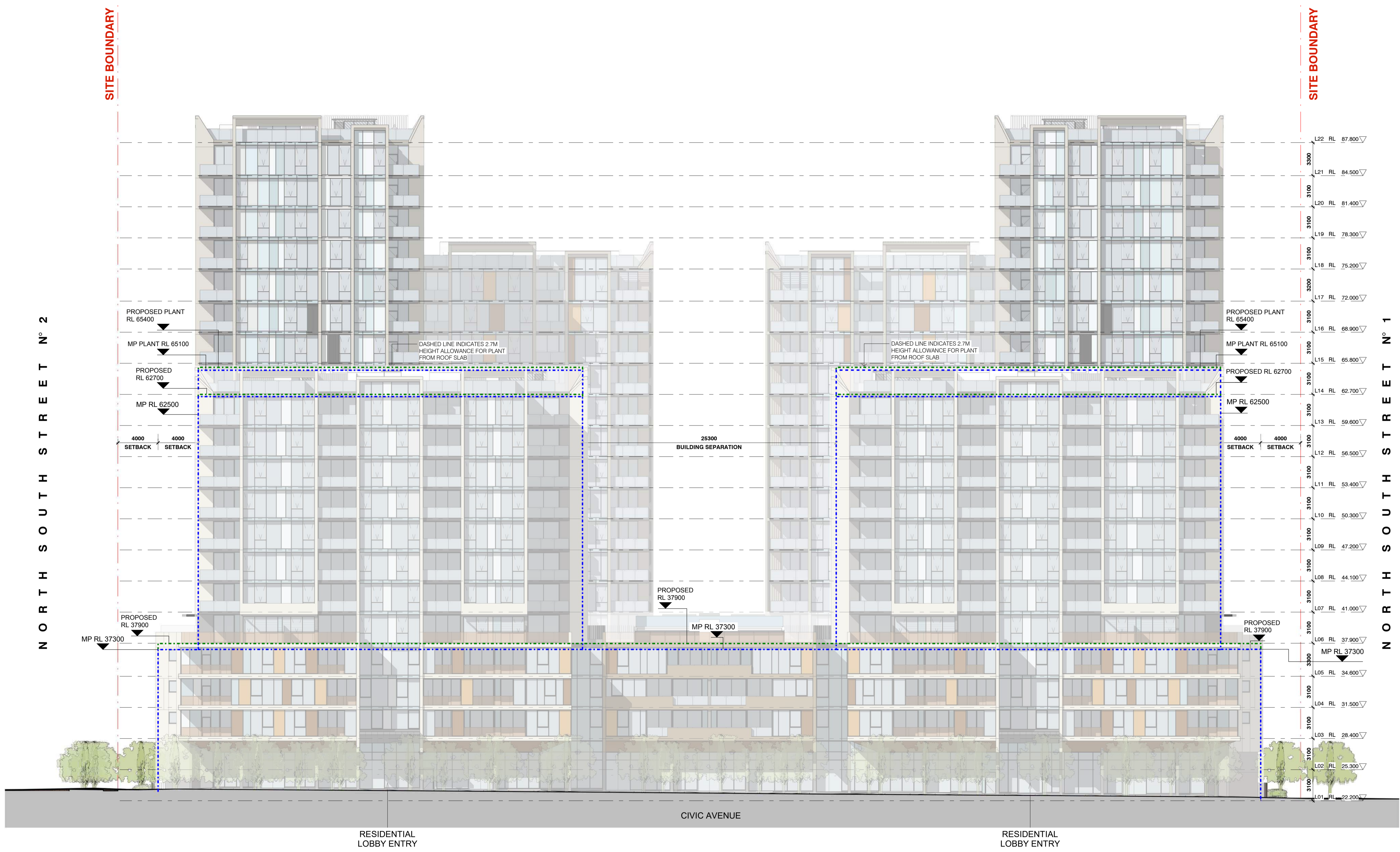
1 ELEVATION - NORTH 1 : 200
